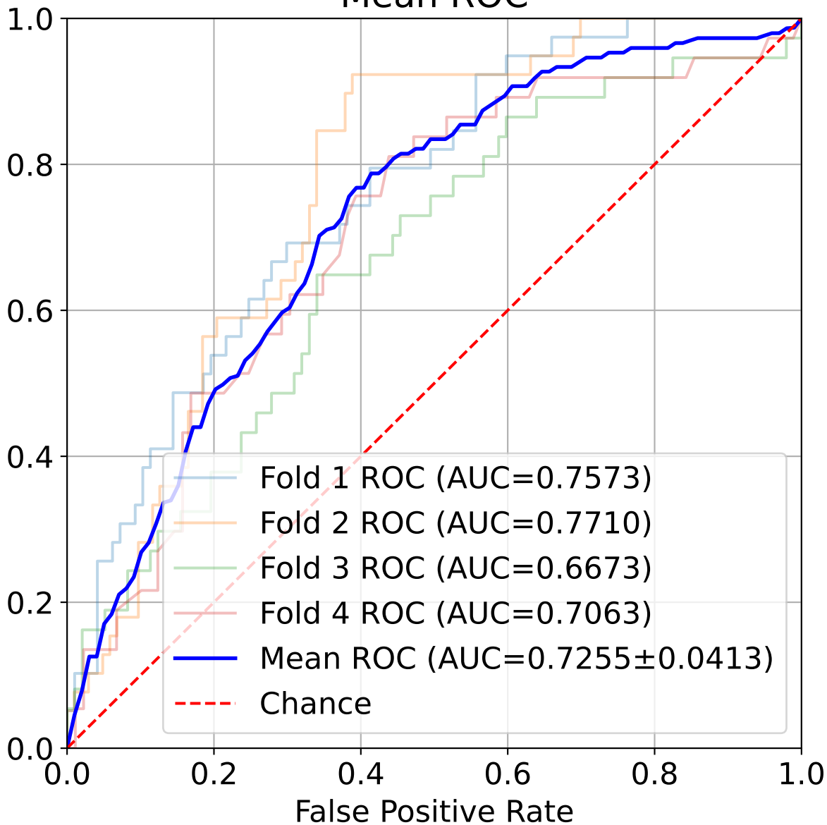
Mean ROC
